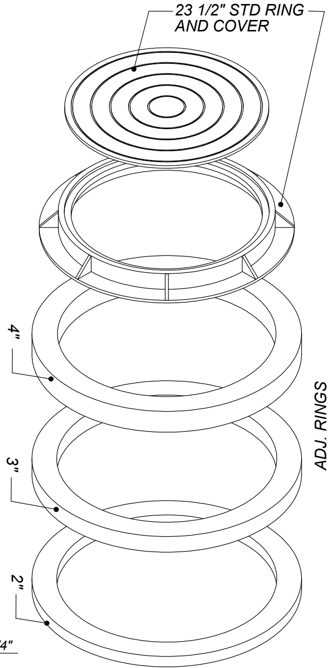
ISOMETRIC
